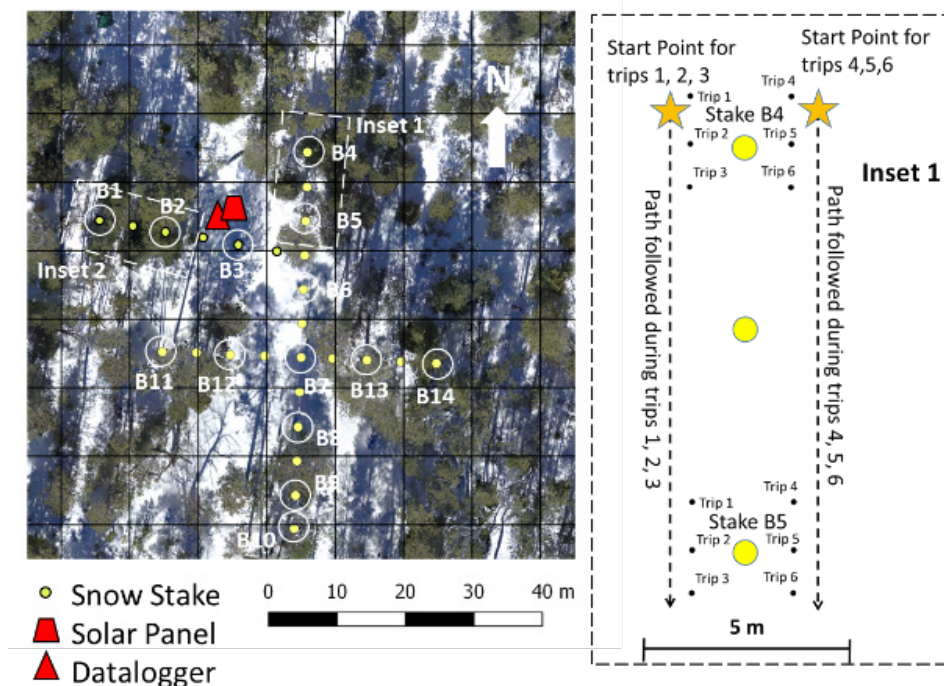
Figure 36. Map of an example snowtopography transect survey showing the locations of snow density samples and the sampling protocol. Source: Patrick Broxton.
