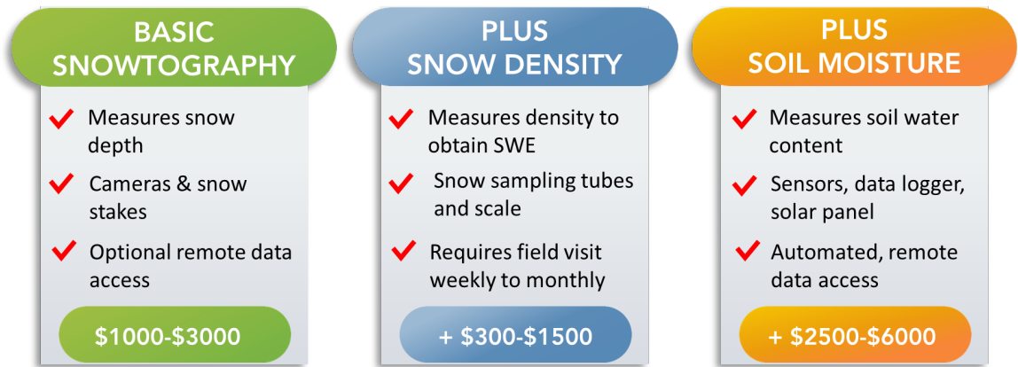
Figure 6. Key elements of the three methods. Dollar amounts are equipment cost estimates and do not include labor or travel costs.
