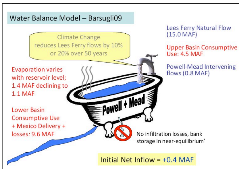
Figure 1. Schematic of simplified water balance model, and assumptions regarding inflows and depletions, used in Barsugli09. The model used in Rajagopalan09 is very similar except that the “bathtub” is larger (60 MAF vs. 50 MAF). See Tables 2 and 3 for a complete list of the model assumptions in these studies and the Barnett studies.
