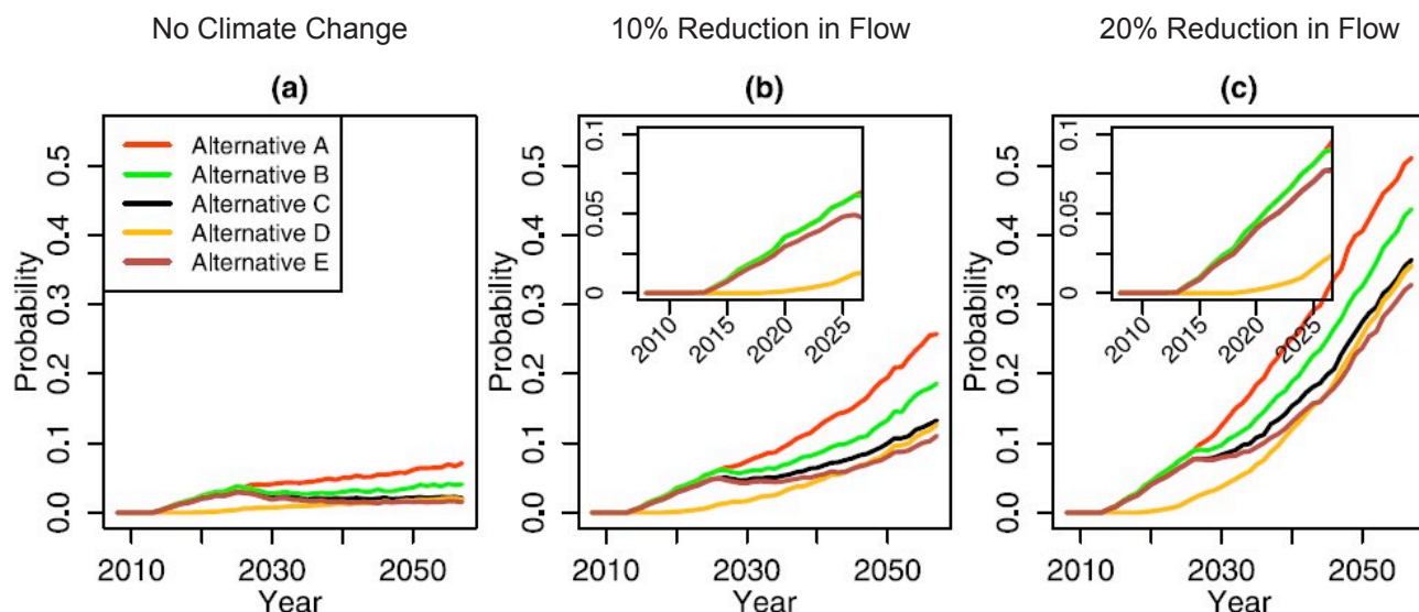
Figure 2. From Rajagopalan09: (a) Risk of drying (depleting system-wide active storage in a given year) for five management alternatives, with an initial demand of 13.5 MAF and no climate change-induced reduction in flow. (b) Same as Figure 2a but for 10% reduction in the annual average inflow over the 50-year period. Inset shows the risk in the near term for the period 2008–2026. (c) Same as Figure 2b but for 20% reduction in annual average inflow. Note: Alternative A (red line) is the current policy (2007 interim shortage guidelines). See Rajagopalan09 for descriptions of all five alternatives.
